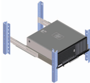
Figure 3. HP xw4/Z2/Z4 Adjustable Sliding Rail Rack Kit—with workstation installed
